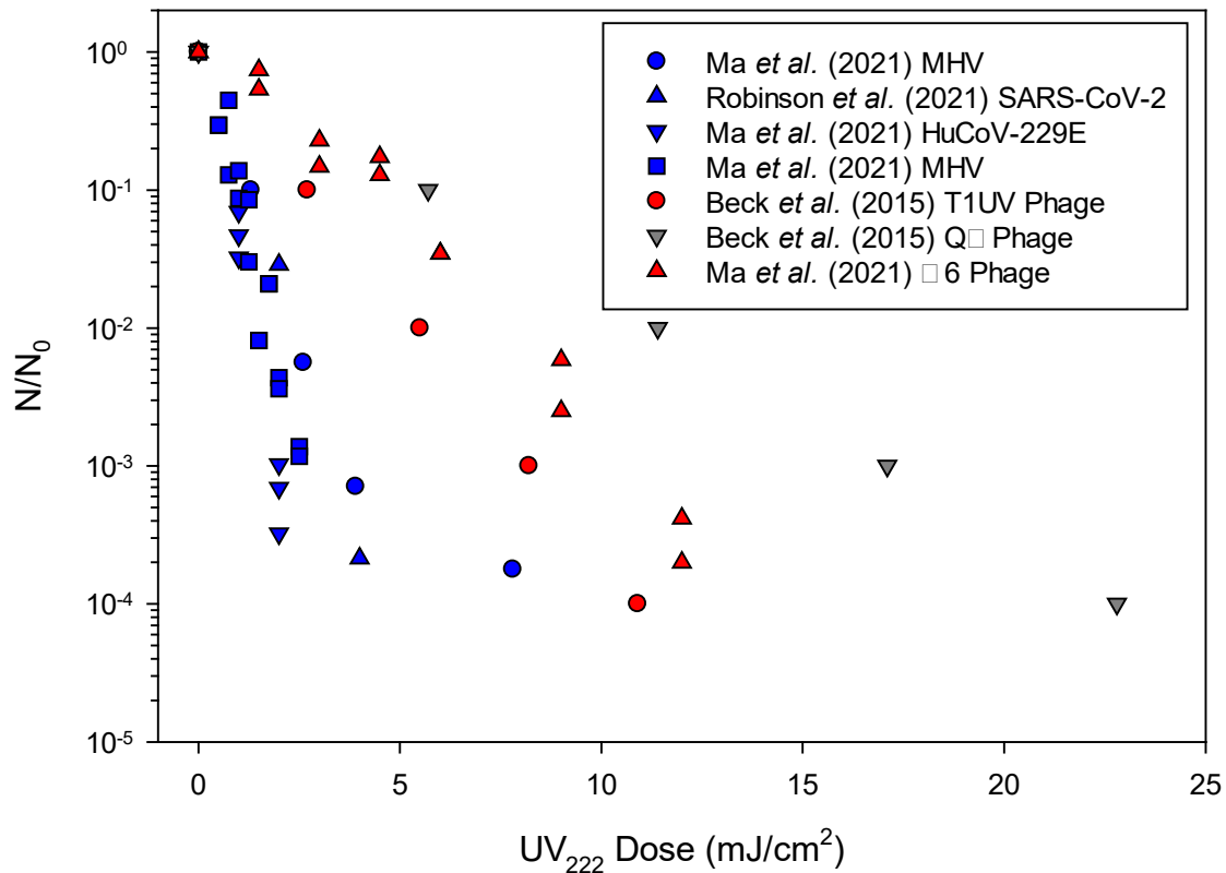
Figure 9. UV 222 dose-response behavior of coronaviruses and phage that could serve as (conservative) surrogates. 13, 19, 25 Measured inactivation responses of coronaviruses are indicated by blue symbols; measured inactivation responses of potential phage surrogates are indicated by red symbols; measured inactivation responses of conservative phage surrogates are indicated by charcoal gray symbols.
