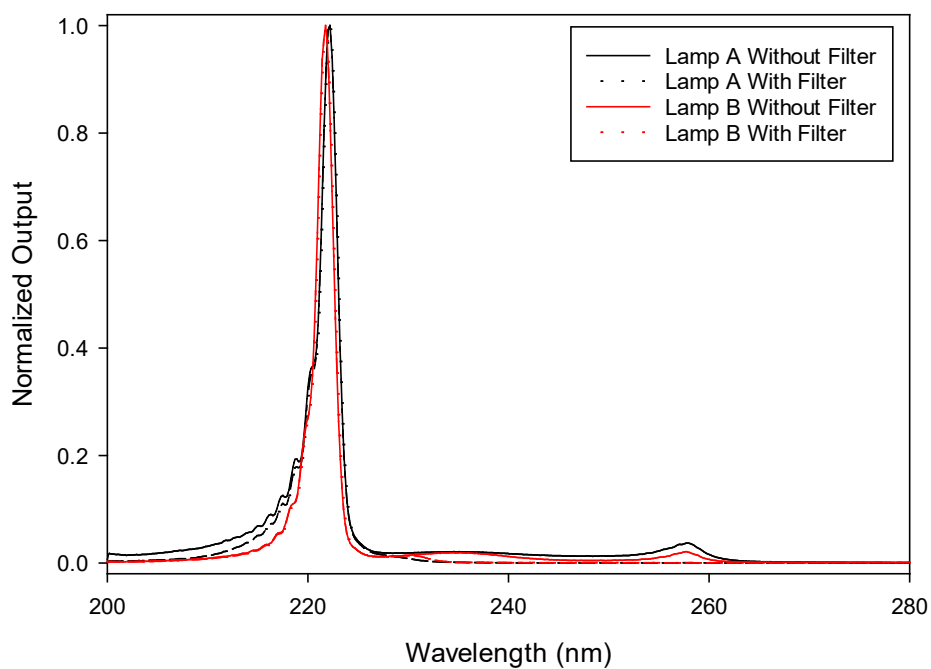
Figure 2. Emission spectra from commercially-available \text{KrCl}^* lamps with and without optical filters. Normalized output presented on a \log_{10} scale (top panel) and on a linear scale (bottom panel). For both lamps, the spectra were measured independently and normalized to output at the wavelength corresponding to peak output ( ca. 222 nm).
