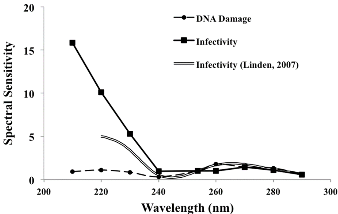
Figure 6. Spectral sensitivity of adenovirus 2 as measured by infectivity, compared to nucleic acid (DNA) damage, for wavelengths between 210 and 290 nm. 28
