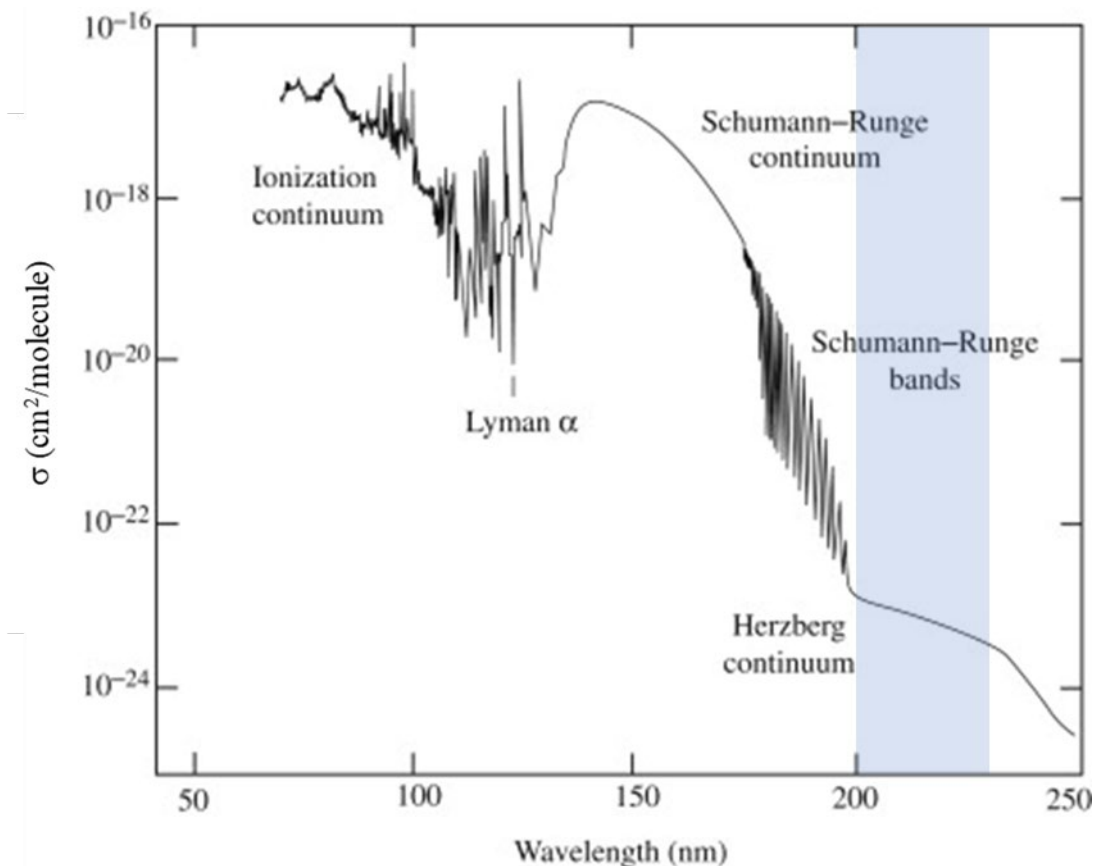
Figure 15. Absorption cross sections for molecular oxygen ( \text{O}_2 ) for wavelengths that comprise the VUV and UV-C ranges. Image modified from Encyclopedia of Atmospheric Sciences . 90 The shaded blue area indicates the Far UV-C range.
