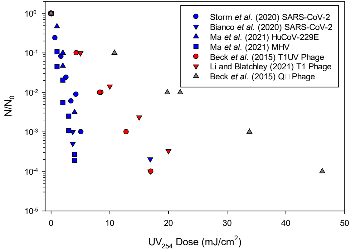
Figure 8. UV 254 dose-response behavior of coronaviruses and phage that could serve as (conservative) surrogates. 13, 17-19, 53 Measured inactivation responses of coronaviruses are indicated by blue symbols; measured inactivation responses of potential phage surrogates are indicated by red symbols; measured inactivation responses of conservative phage surrogates are indicated by charcoal gray symbols.
