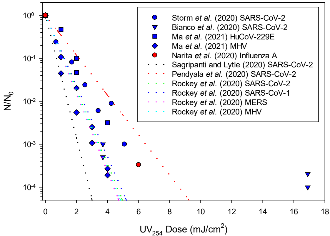
Figure 4. Measured UV_{254} dose-response behavior of common ssRNA respiratory pathogens, including numerous coronaviruses, in aqueous suspension. 17-20 Measured inactivation responses of coronaviruses are indicated by blue symbols; measured inactivation of Influenza A virus is indicated by red symbols. Also included are predictions of coronavirus responses from genomic models (dashed lines). 21-23
